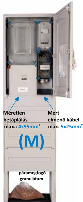
GYI53-63-SK95/SK-(M) GYI53-80-SK95/SK-(M)
