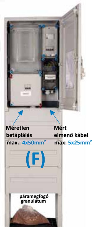
GYI53-63-SK50/SK-(F) GYI53-80-SK50/SK-(F)
