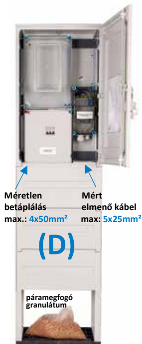
GYI53-63-SK50/SK-(G) GYI53-80-SK50/SK-(G)
