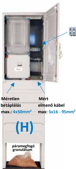
GYI53-63-SK50/SK-(H) GYI53-80-SK50/SK-(H)
