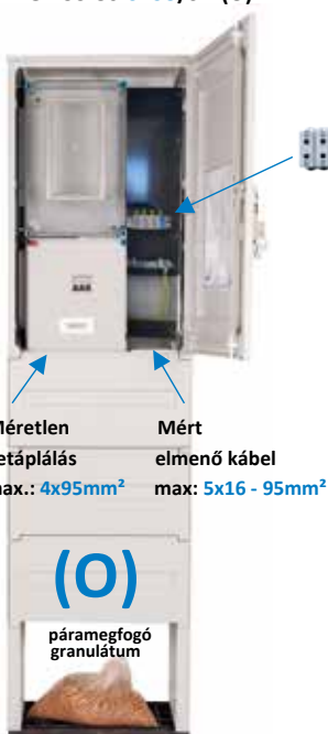
GYI53-63-SK95/SK-(O) GYI53-80-SK95/SK-(O)
